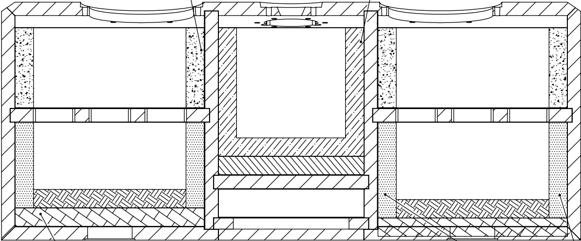
SECTION VIEW A
